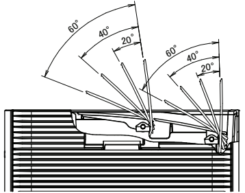
Horizontal blade movable range
